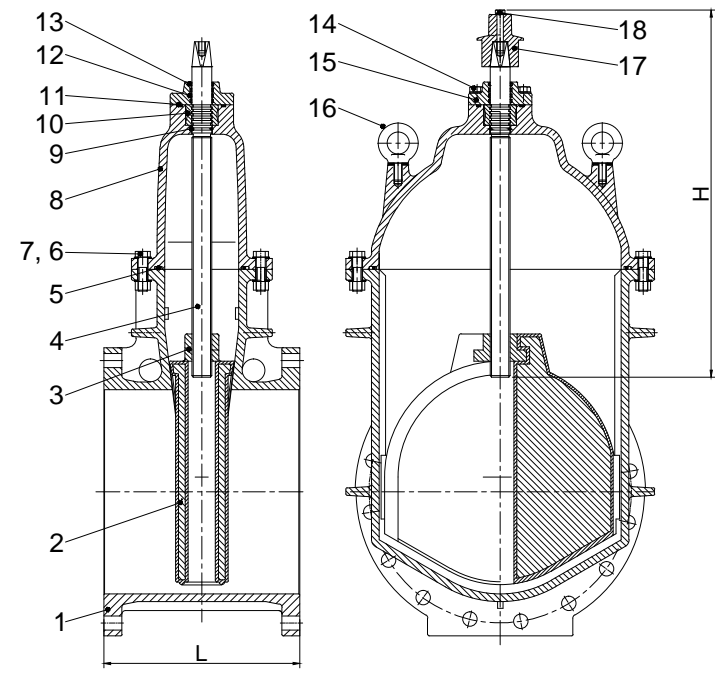
Dimensions-inch
